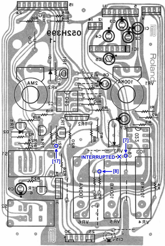
ROLAND SH-101 Bender Board OPH178-1 (view from foil side)
